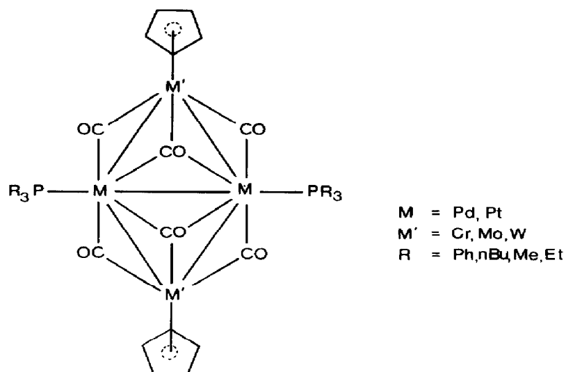
Fig. 3. The planar clusters [M_2M'_2(\text{CO})_6(\eta^5\text{-C}_5\text{H}_5)_2(\text{PR}_3)_2] .
